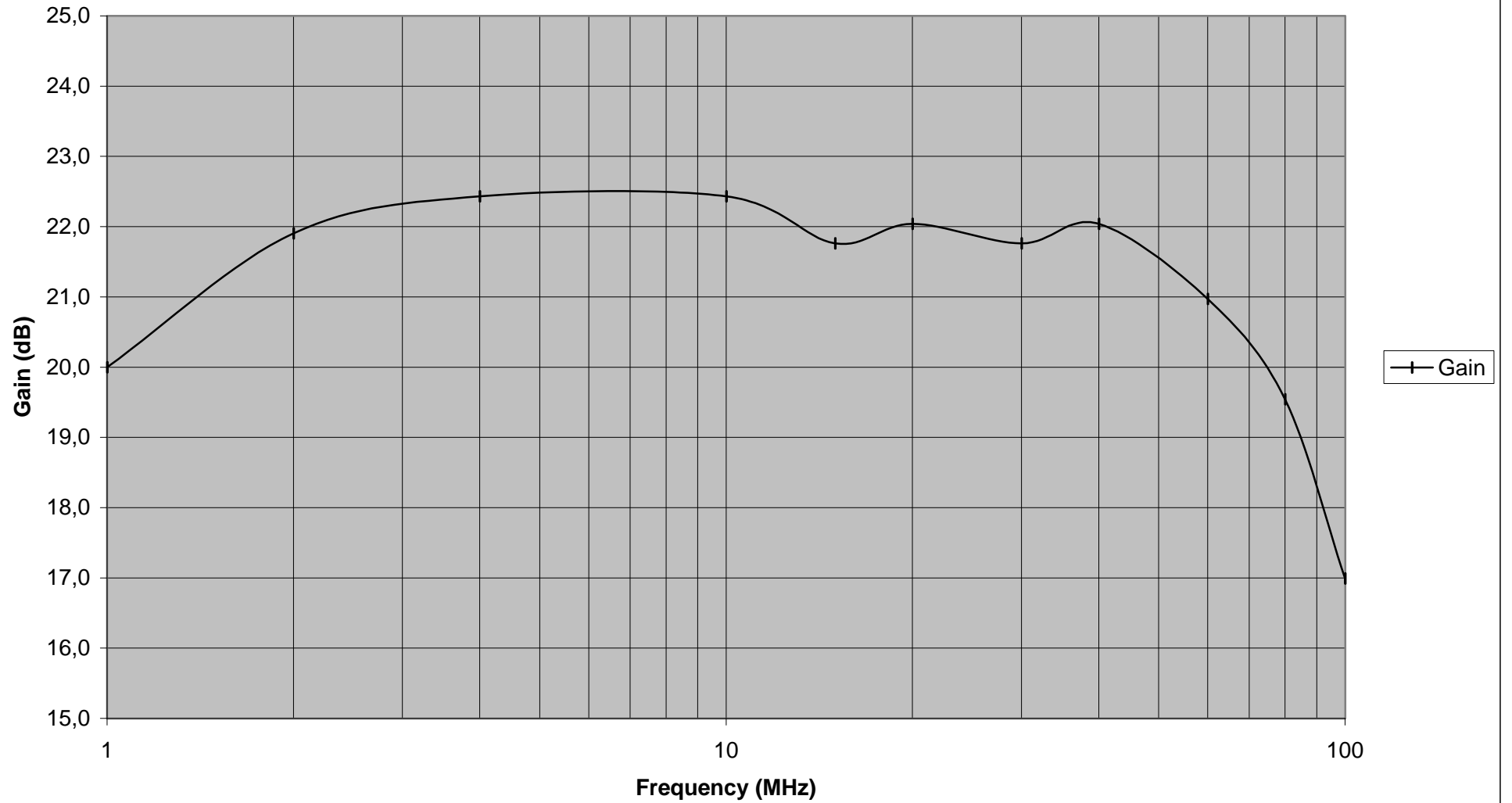
10W Amp Gain versus Freq
