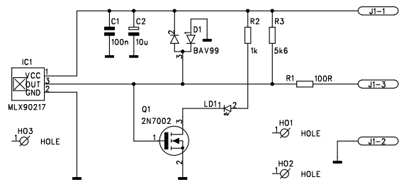
CAM Sensor
