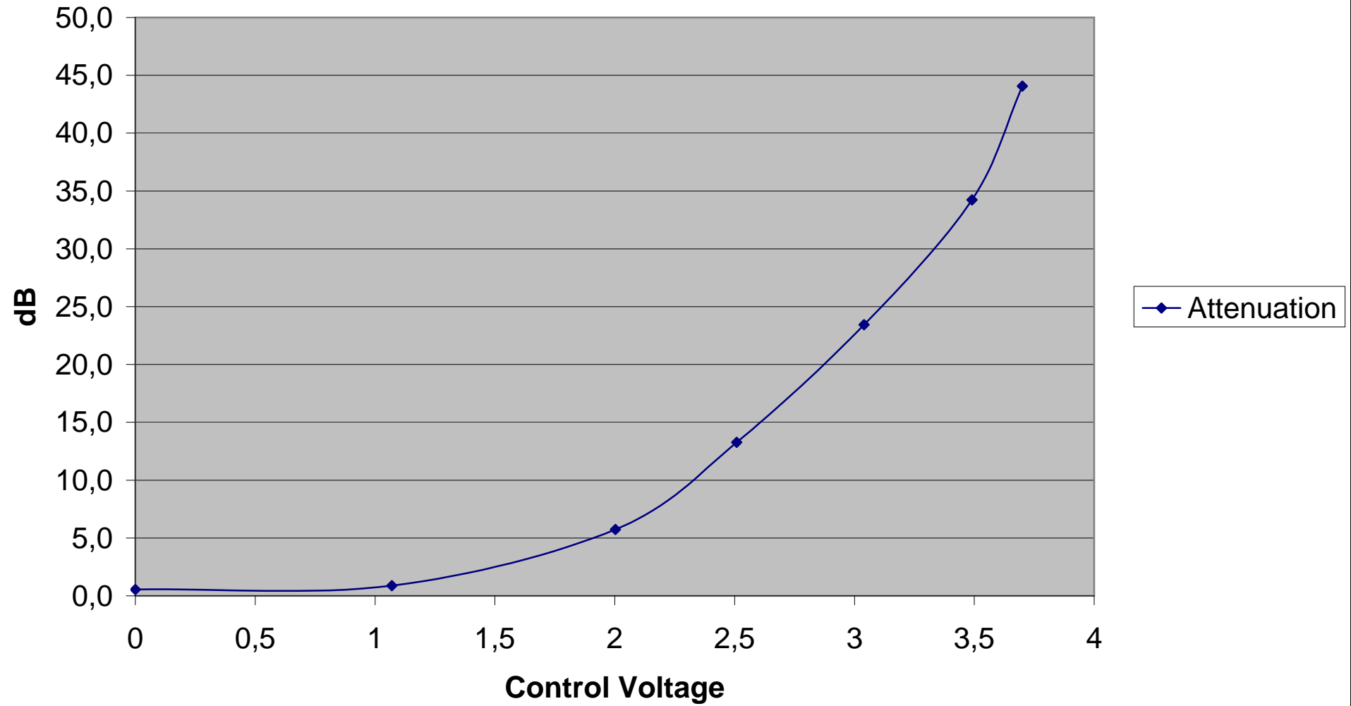
OH2NLT RF diode attenuator
